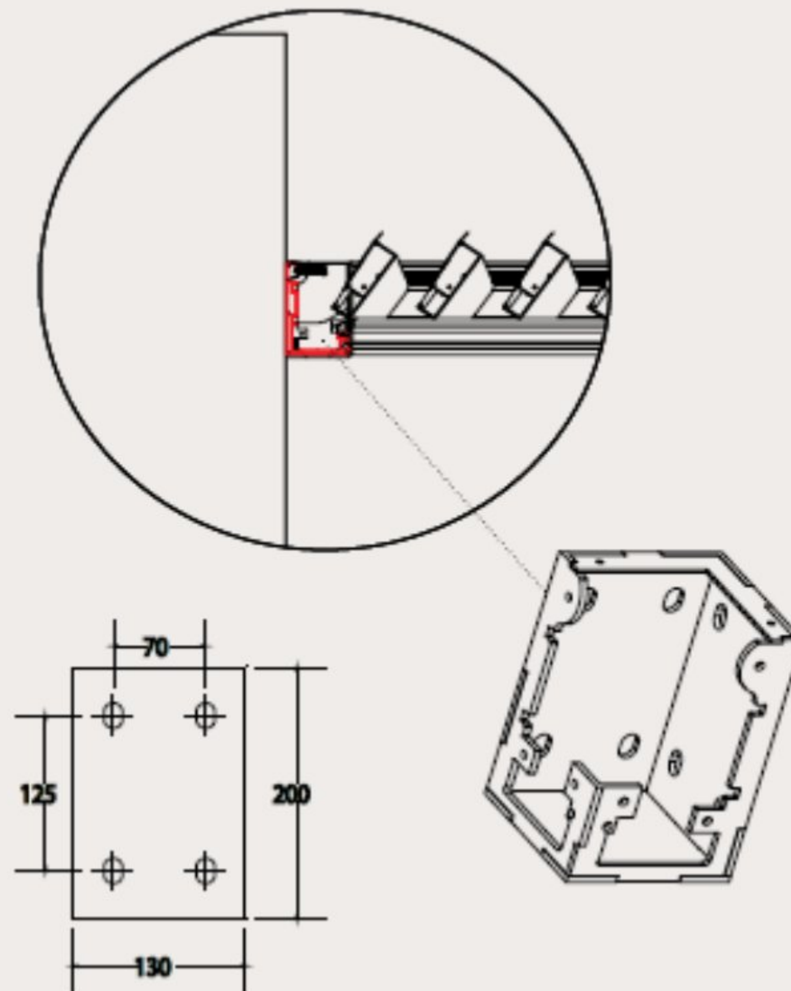
Wall base detail
