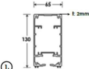
1. Side Guides
