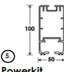
5. Powerkit Support Profile
