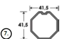
7. Int. Tube Drive Shaft profile
