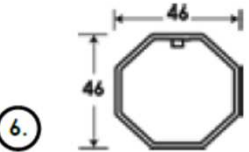
6. Ext. Tube Drive Shaft Profile
