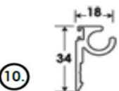
10. Jolly Cloth Profile
