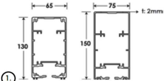
1. Side Guides
