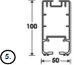
5. Powerkit Support Profile
