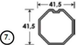
7. Int. Tube Drive Shaft profile
